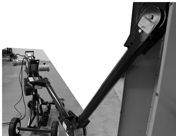
Down Pull using elbow unit and nose unit with 45° horizontal pivot feature
