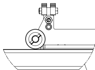
Hinged conduit support block in raised position
